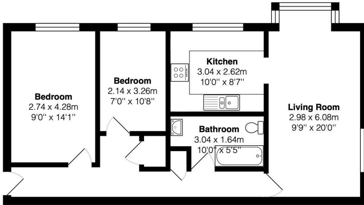
Second Floor Area: 62.7 m 2 ... 675 ft 2
