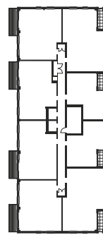
FOURTH FLOOR
